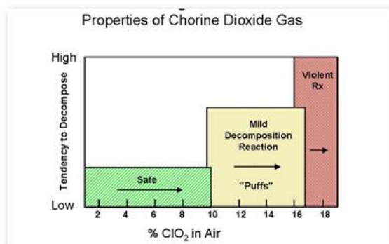
Figure 1: Properties of Chlorine Dioxide Gas
