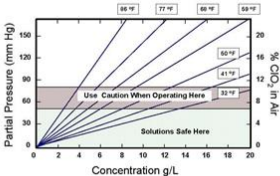
Figure 2: Partial Pressures in Solution
